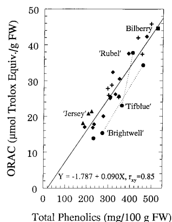
Figure 2. Relationship between total phenolic concentrations ( X ) (mg/100 g of fresh weight) to ORAC ( Y ) ( \mu\text{mol} Trolox equiv/g of fresh berry) in different cultivars of Vaccinium species ( Y = -1.787 + 0.090X ; r_{xy} = 0.845 ; n = 28 ). \blacklozenge , Vaccinium corymbosum L. (Highbush); \blacktriangle , cv. Jersey (highbush); + , Vaccinium angustifolium Ait. Lowbush; \blacksquare , Vaccinium myrtillus L. (bilberry); \bullet , Rabbiteye. Data for the two points for the early and late harvest dates for cv. Tifblue and cv. Brightwell are connected by a line.
