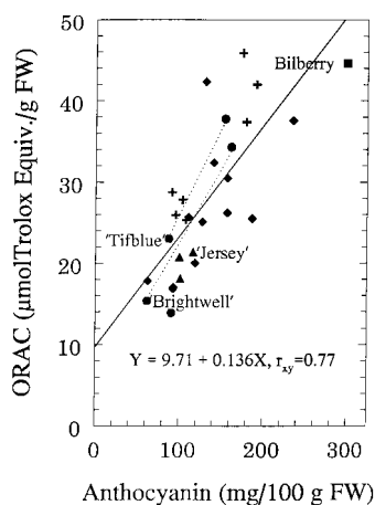
Figure 1. Relationship between anthocyanin concentrations ( X ) (mg/100 g of fresh weight) to ORAC ( Y ) ( \mu\text{mol} Trolox equiv/g of fresh berry) in different cultivars of Vaccinium species ( Y = 9.71 + 0.136X ; r_{xy} = 0.77 ; n = 28 ). \blacklozenge , Vaccinium corymbosum L. (highbush); \blacktriangle , cv. Jersey (Highbush); + , Vaccinium angustifolium Ait., Lowbush; \blacksquare , Vaccinium myrtillus L. (bilberry); \bullet , Rabbiteye. Data for the two points for the early and late harvest dates for cv. Tifblue and cv. Brightwell are connected by a line.
